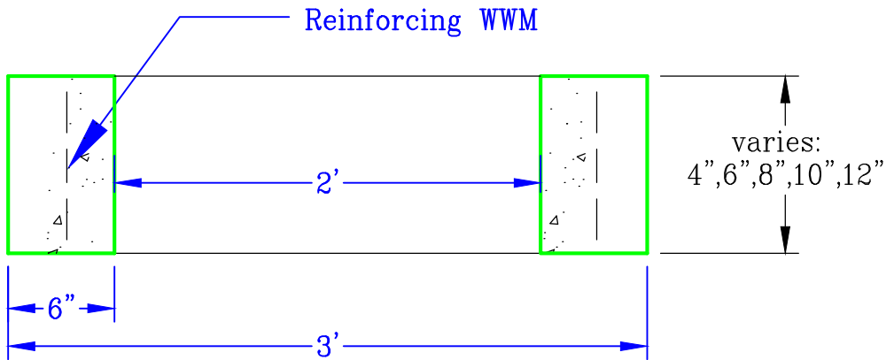
SECTION
